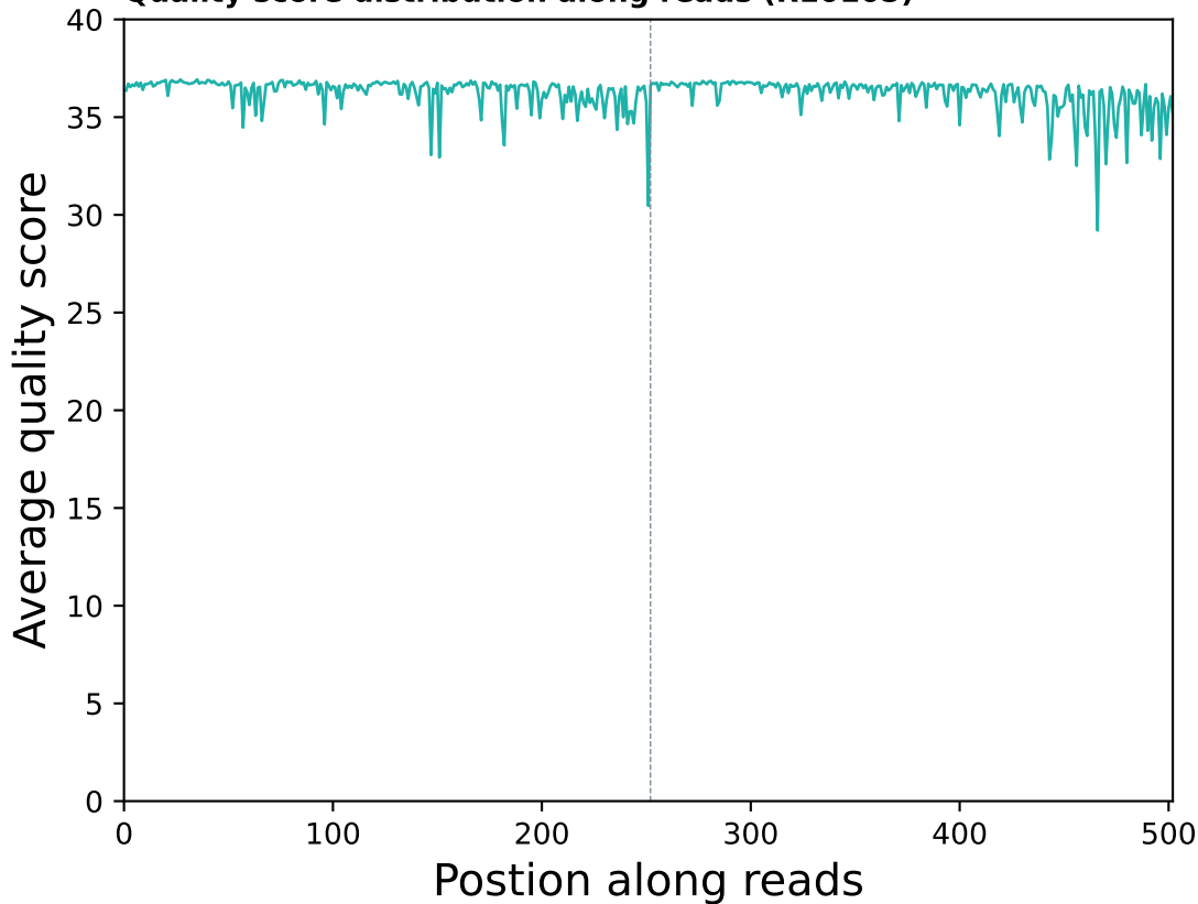
Quality score distribution along reads (R10105)
